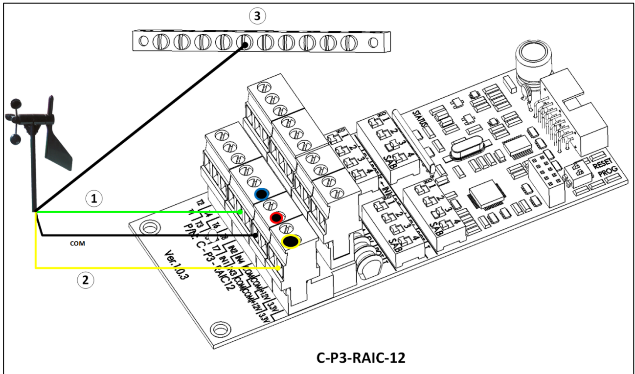
Figure 1: Wind diection sensor wiring
