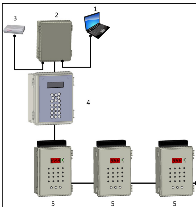
图 1: Super Guard - Pig Guard Plus - Communication Box 联网示意图
